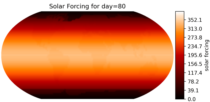
Figure 3: Example plot for the solar forcing on day 80 of the year
