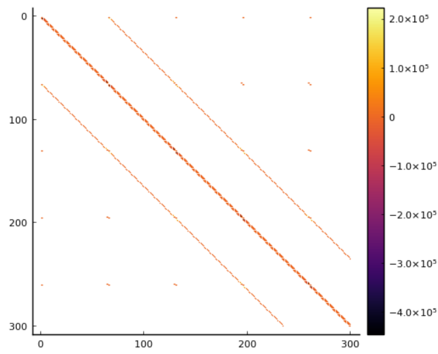
Figure 2: Sparsity pattern of the upper left part of the system matrix
