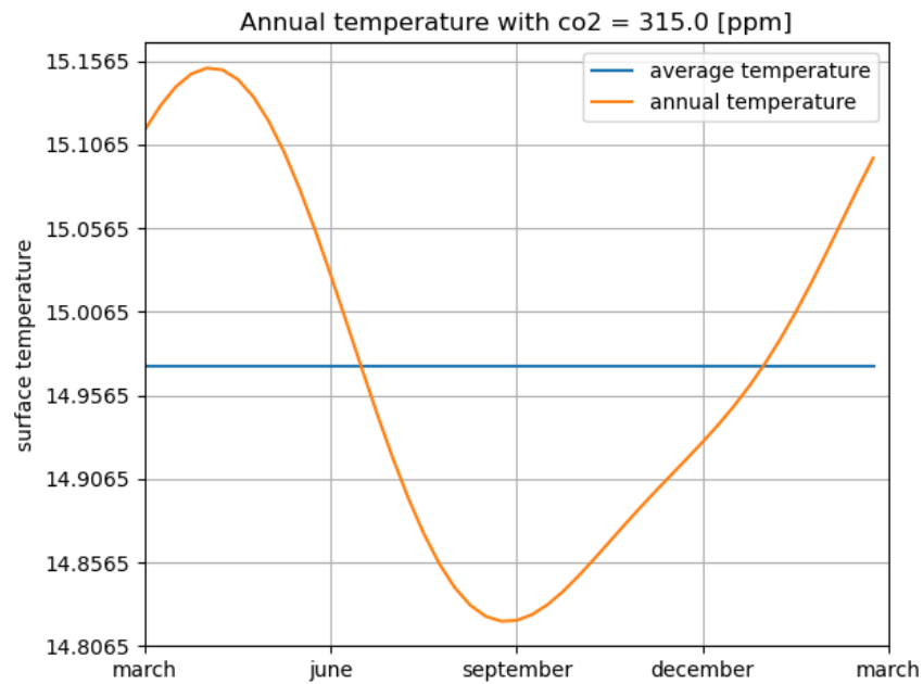
Figure 1: EBM results calculated with forward Euler method (results calculated with backward Euler method are similar)
