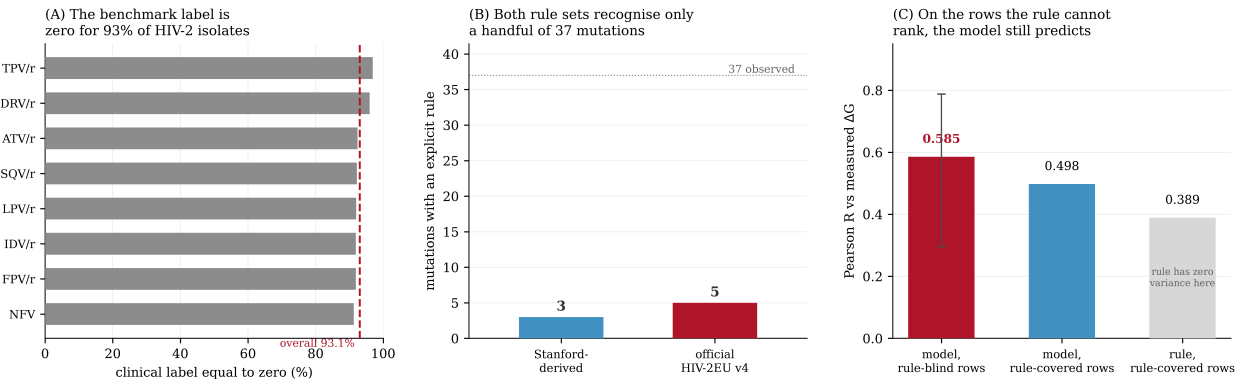
Figure 8. Rule-based HIV-2 interpretation covers only a small fraction of sequence space. (a) The clinical benchmark label is zero for 93.1% of isolates (91.3–96.9% across eight protease inhibitors); the dashed line marks the overall value. (b) Of the 37 distinct mutations present in the measured ChEMBL panel, the Stanford-derived rule table recognises three (blue) and the official HIV-2EU v4 rules five (red), against 37 observed (dotted line). (c) On the 116 measured rows where the rule score is zero—and therefore carries no ranking
