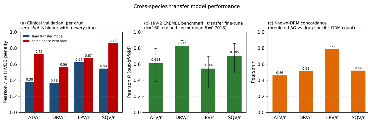
Figure 9. Cross-species transfer model performance. (a) Per-drug external clinical validation: Pearson correlation between predicted binding free energy and the Stanford HIVDB penalty score for the final transfer model (blue) and the same-space zero-shot baseline (red); within every drug the zero-shot baseline is higher, so no per-drug clinical superiority of the transfer fine-tune is claimed. (b) HIV-2 ChEMBL out-of-fold benchmark for the transfer fine-tune (n=160; error bars 95% percentile-bootstrap CI; dashed line, mean R=0.7018). (c) Known-drug-resistance-mutation concordance: Pearson correlation between predicted binding free energy and the drug-specific DRM count per sequence. All values are read directly from the locked result manifest.
