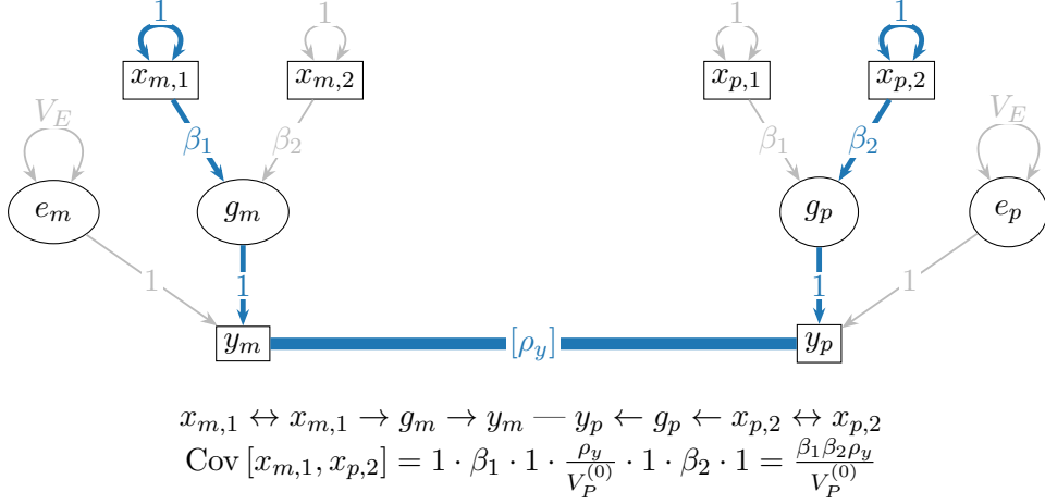
Figure 1: A mated pair in the base population, assorting on the phenotype with strength \rho_y , with one chain traced on it and the product of its coefficients written underneath. The trait is built from two causal variants, g_i = \beta_1 x_{i,1} + \beta_2 x_{i,2} , and each individual's phenotype is y_i = g_i + e_i . Genotypes and phenotypes are observed (rectangles); genetic and environmental values are latent (ellipses). Self-loops are exogenous variances: each standardized genotype has variance 1 and each environmental deviation has variance V_E . The single thick line is the co-path, labelled with the correlation it induces. The edges the chain does not use are faded rather than omitted, so the figure still states the whole model and any other covariance can be traced off the same picture.
