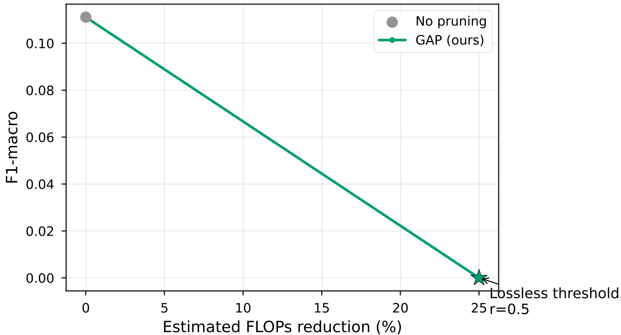
Accuracy-FLOPs Pareto
