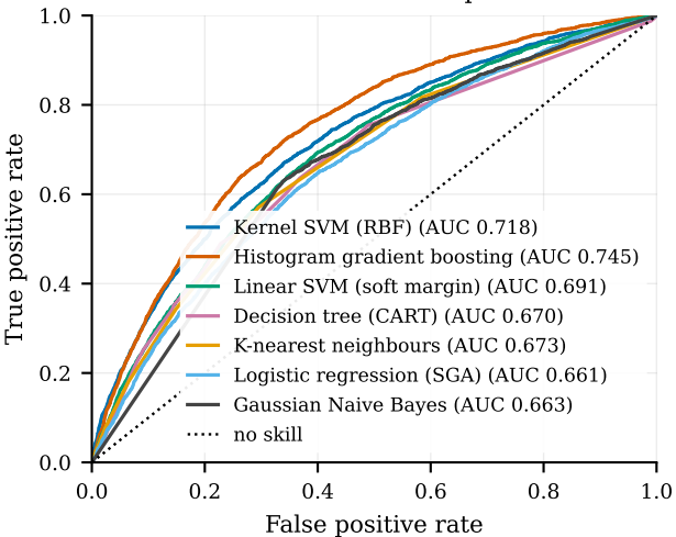
ROC on the test split
