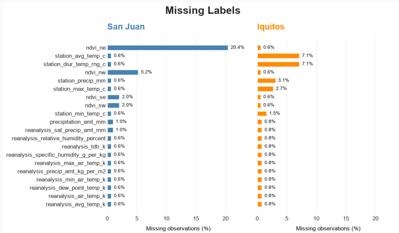
Figure 4: Missing values by column and city
