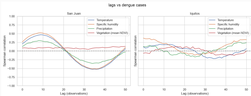
Figure 5: Spearman correlation of lagged weather with current cases
