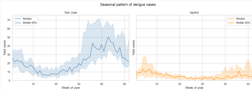
Figure 2: Seasonal profile: median cases by week of year
