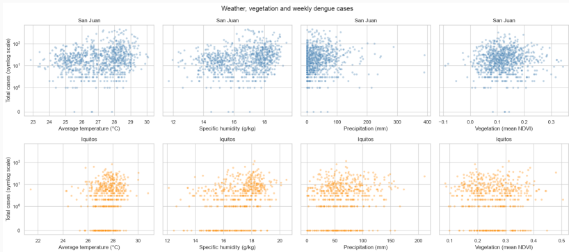
Figure 3: Weather and vegetation against case counts
