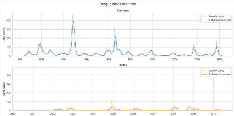
Figure 1: Weekly dengue cases over time, by city
