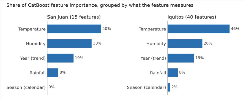
Figure 2: CatBoost feature importance by feature family
