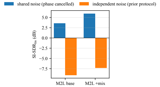
Fig. 2. Decode-noise protocol confound (Music2Latent, MUSDB18, \alpha=0.5 ). The same checkpoints score deeply negative under independent-noise decoding and positive under shared-noise decoding; the negative scores reflect decoder noise, consistent with phase variance, not latent linearity.
