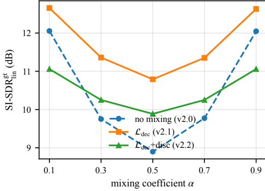
Fig. 3. Ground-truth equivariance vs. mixing coefficient \alpha (source-balanced subsample). The no-mixing baseline sags at the hardest balanced mix ( \alpha=0.5 ); the decode-mixing loss flattens and lifts the curve across all \alpha .
