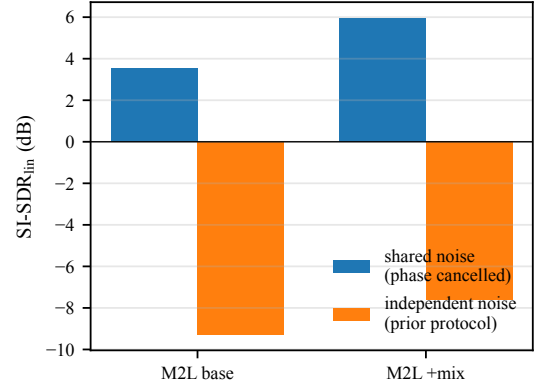
Fig. 1. Decode-noise protocol confound (Music2Latent, MUSDB18, \alpha=0.5 ). The same checkpoints score deeply negative under independent-noise decoding and positive under shared-noise decoding; the \approx -8 dB figure is a phase artifact, not a linearity measurement.
