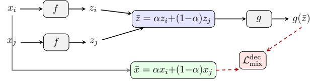
Fig. 2. Decode-mixing loss: encode a pair, interpolate latents, decode, and compare to the true waveform mix. Gradients (dashed) flow through the decoder and back into the encoder via \bar{z} .
