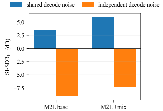
Fig. 2. Decode-noise protocol confound (Music2Latent, MUSDB18, \alpha=0.5 ). The same checkpoints score deeply negative under independent-noise decoding and positive under shared-noise decoding; the negative scores reflect decoder sampling noise rather than latent linearity.
