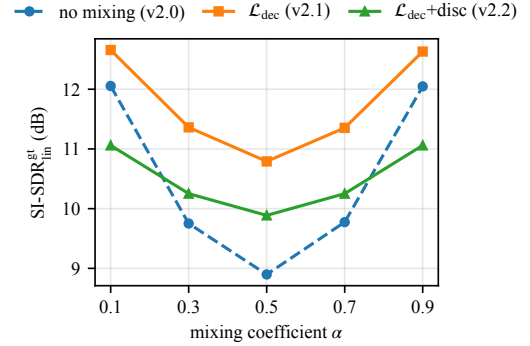
Fig. 3. Ground-truth equivariance vs. mixing coefficient \alpha (source-balanced subsample). The no-mixing baseline sags at the hardest balanced mix ( \alpha=0.5 ); the decode-mixing loss flattens and lifts the curve across all \alpha .
