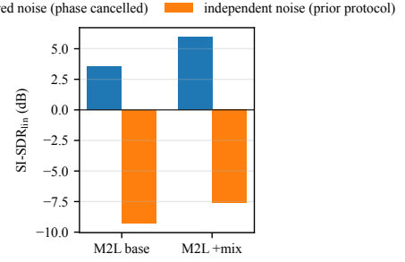
Fig. 1. Decode-noise protocol confound (Music2Latent, MUSDB18, \alpha=0.5 ). The same checkpoints score deeply negative under independent-noise decoding and positive under shared-noise decoding; the \approx -8 dB figure reflects decoder noise, consistent with phase variance, not latent linearity.
