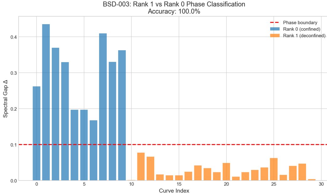
Figure 3: BSD-003: Rank 1 vs Rank 0 . Clear phase separation: rank-0 curves have \Delta > 0 (confined), rank-1 curves have \Delta \approx 0 (deconfined).
