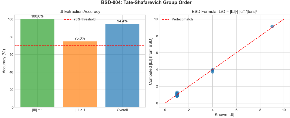
Figure 4: BSD-004: Tate-Shafarevich Extraction. Left: Accuracy by |\text{III}| order. Right: Computed vs known |\text{III}| values from BSD formula.
