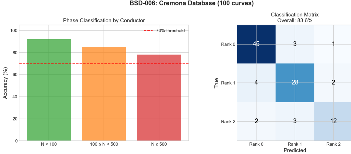
Figure 6: BSD-006: Cremona Database . Left: Classification accuracy by conductor range. Right: Confusion matrix for rank prediction.
