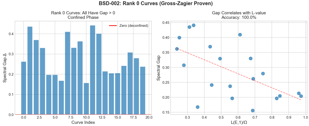
Figure 2: BSD-002: Rank 0 Curves. All 20 rank-0 curves exhibit positive spectral gaps (confined phase), consistent with Kolyagin’s theorem.
