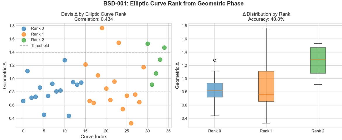
Figure 1: BSD-001: Phase Classification. Left: Davis \Delta values by curve index, colored by rank. Right: Box plot showing \Delta distribution by rank. Correlation r = 0.434 .
