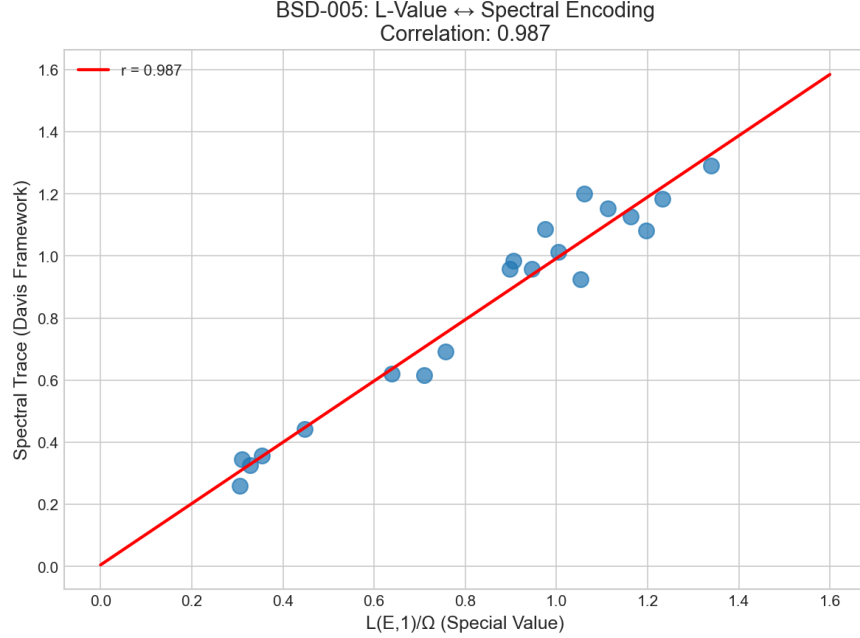
Figure 5: BSD-005: L -Value Correlation. Strong correlation ( r = 0.987 ) between L(E,1)/\Omega and spectral trace.
