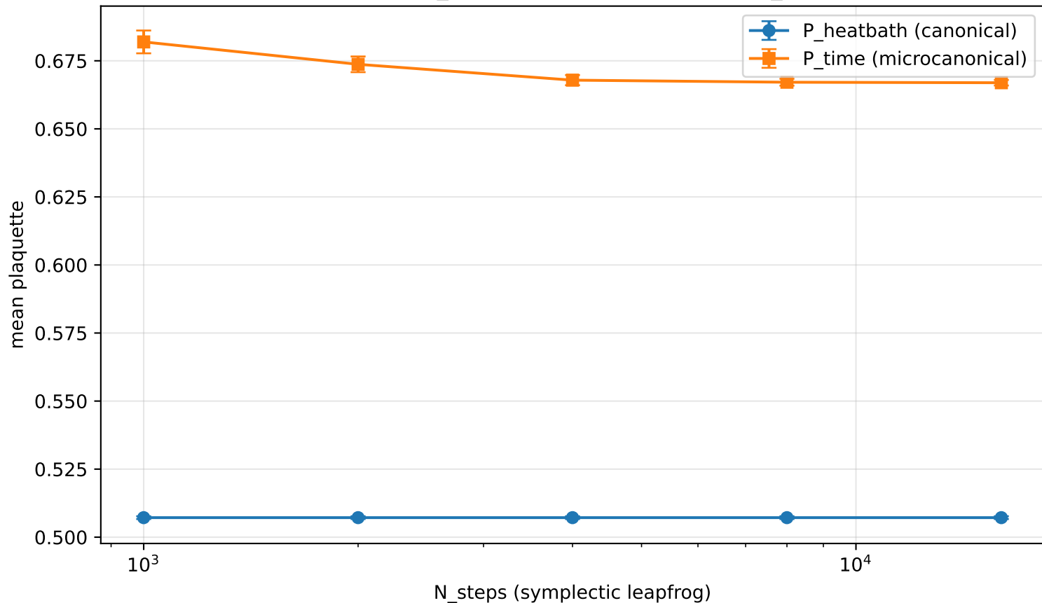
Microcanonical P_time approaches canonical P_heatbath?
