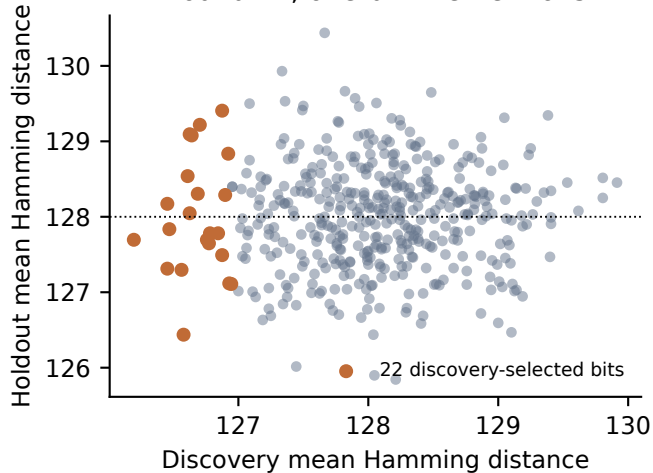
Round 24; one-bit interventions
