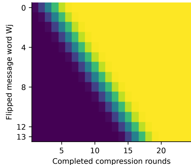
Holdout mean Hamming distance
