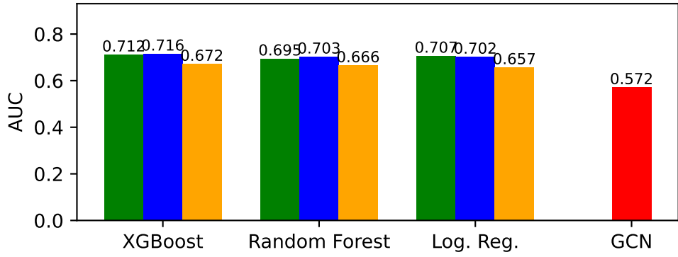
contact-high-school — AUC
