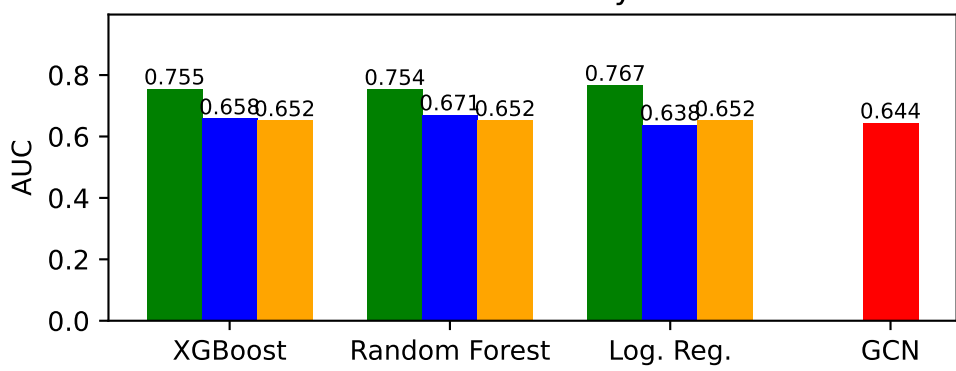
coauth-MAG-Geology — AUC
