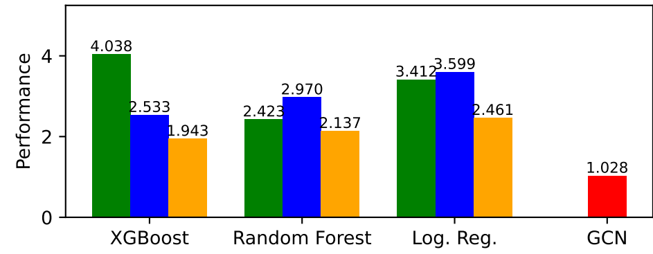
contact-primary-school-2 — Performance
