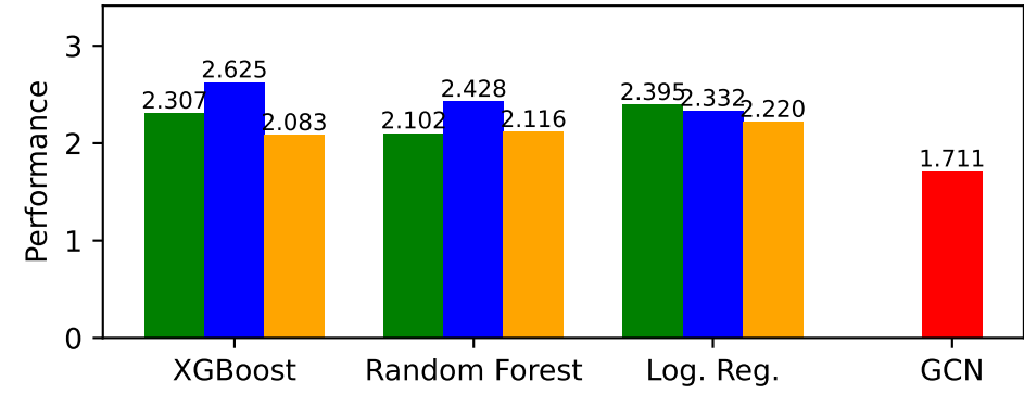
contact-high-school — Performance
