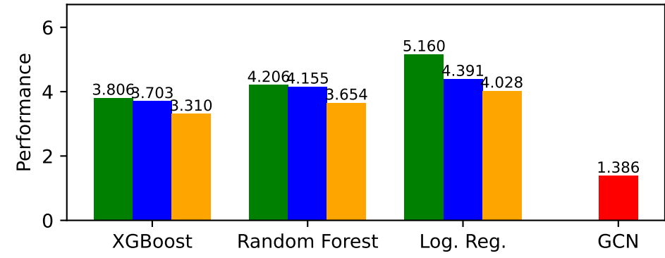
email-Eu — Performance
