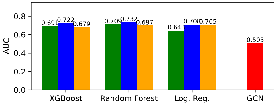
contact-primary-school-2 — AUC
