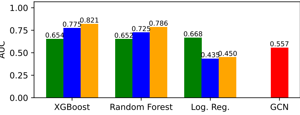
NDC-classes — AUC
