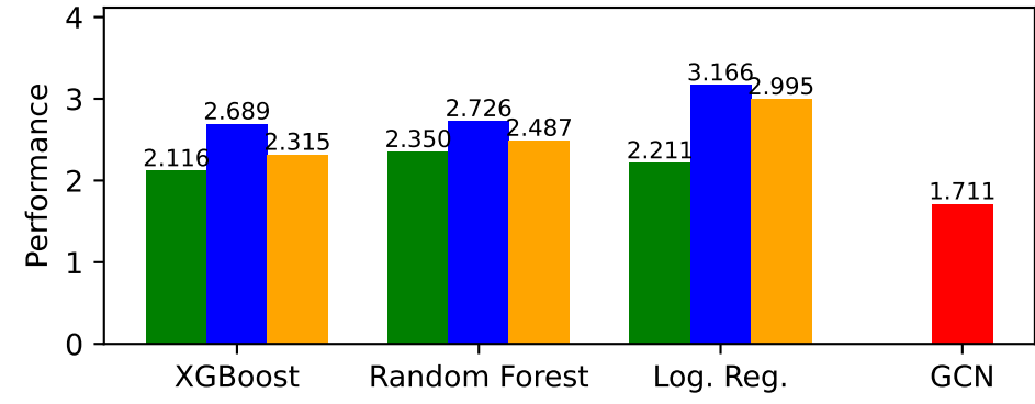
email-Enron — Performance
