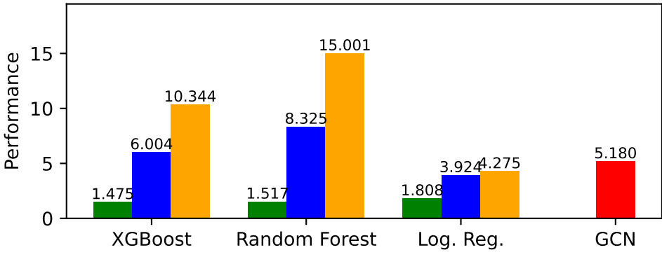
NDC-classes — Performance
