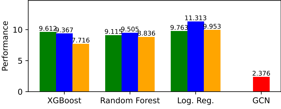
threads-ask-ubuntu — Performance
