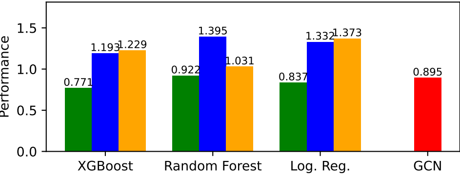
NDC-substances — Performance
