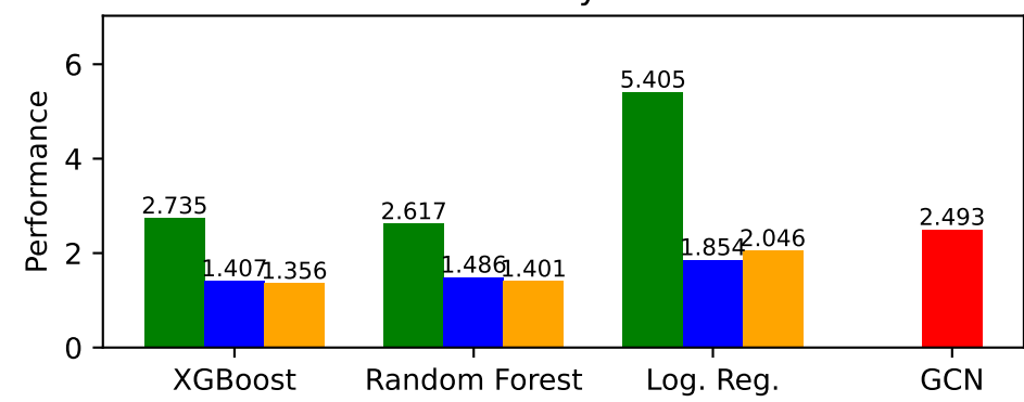
coauth-MAG-Geology — Performance
