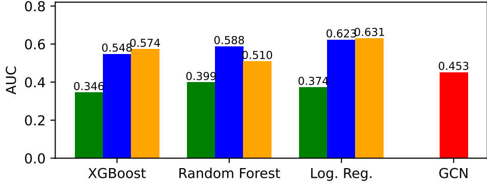
NDC-substances — AUC
