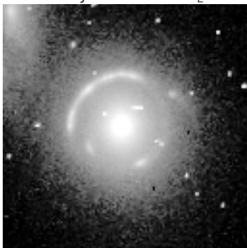
S4TM SDSSJ0753+3416 \theta_E=1.23''
