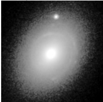
SLACS J0728+3835 \theta_E=1.25''
