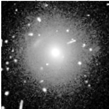
S4TM SDSSJ1553+3004 \theta_E=0.84''
