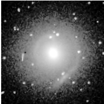
SLACS J1204+0358 \theta_E=1.31''
