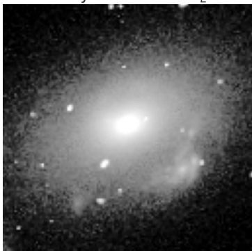
S4TM SDSSJ1048+1313 \theta_E=1.18''
