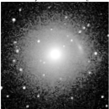
S4TM SDSSJ0754+1927 \theta_E=1.04''
