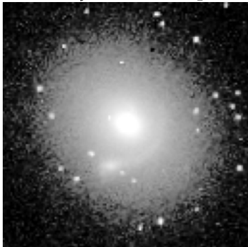
S4TM SDSSJ1144+0436 \theta_E=0.76''
