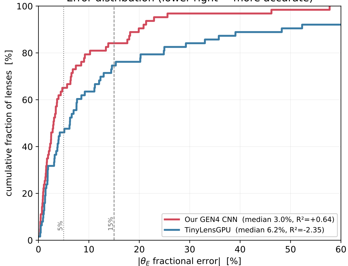
Error distribution (lower-right = more accurate)
