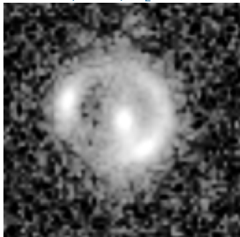
SIM (GEN5) \theta_E=1.24''
