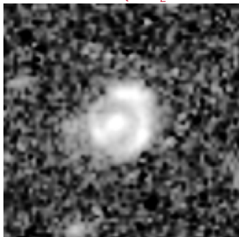
REAL Euclid Q1 \theta_E=0.72''
