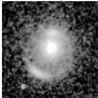
SIM (GEN5) \theta_E=1.43''
