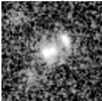
SIM (GEN5) \theta_E=0.72''
