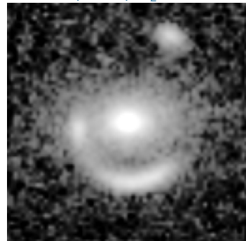
SIM (GEN5) \theta_E=1.83''
