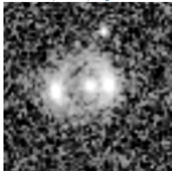
SIM (GEN5) \theta_E=0.94''
