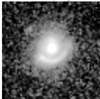
REAL Euclid Q1 \theta_E=0.75''
