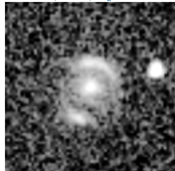
SIM (GEN5) \theta_E=1.04''
