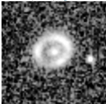
SIM (GEN5) \theta_E=0.85''
