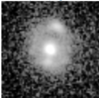
SIM (GEN5) \theta_E=1.15''
