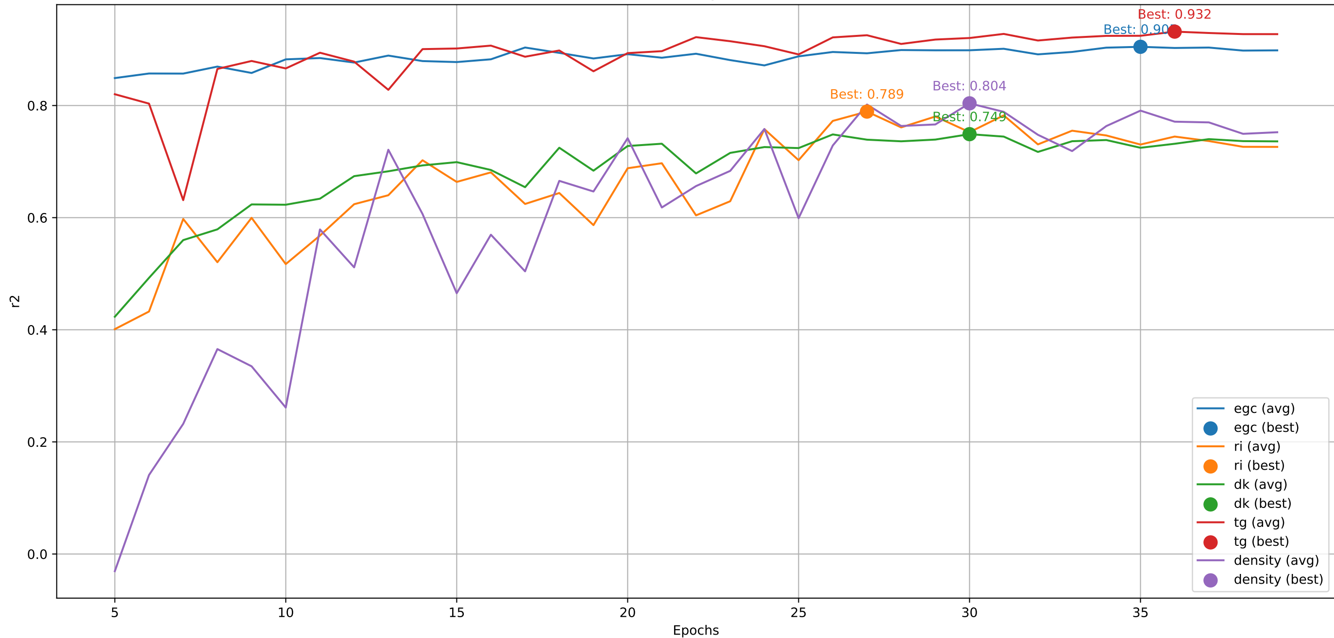
Plot for Metric: r2 (Averages with Best Values)
