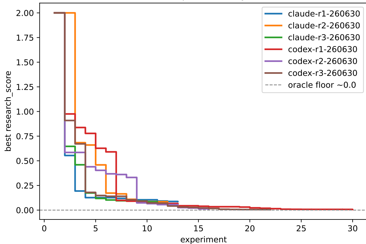
Sample efficiency
