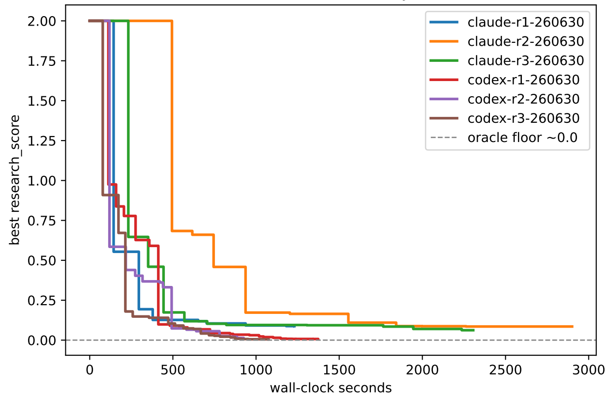
Wall-clock efficiency
