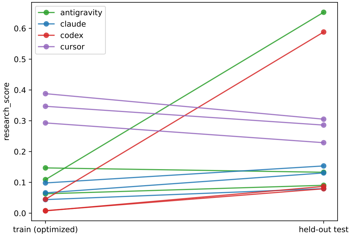
Full research_score (with abstain)
