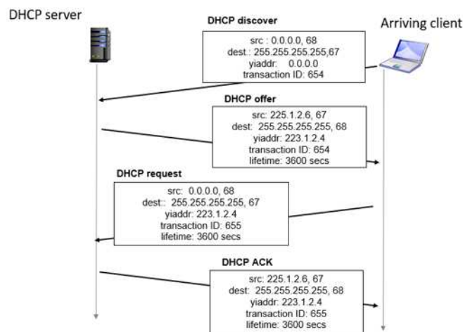
Figure 1: DHCP client-server scenario
