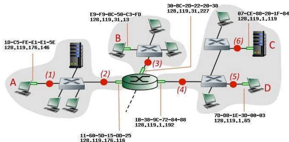
Figure 2: Network Topology for Q.3(b)
