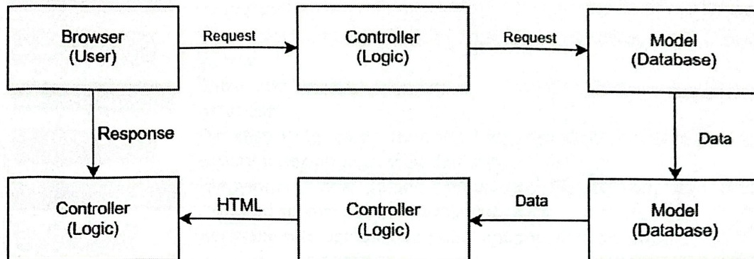
Diagram Alur MVC:
