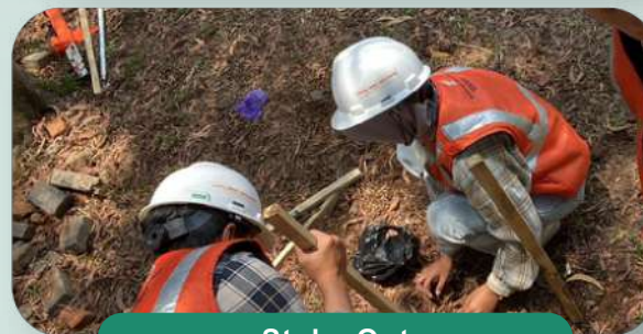
Stake Out
