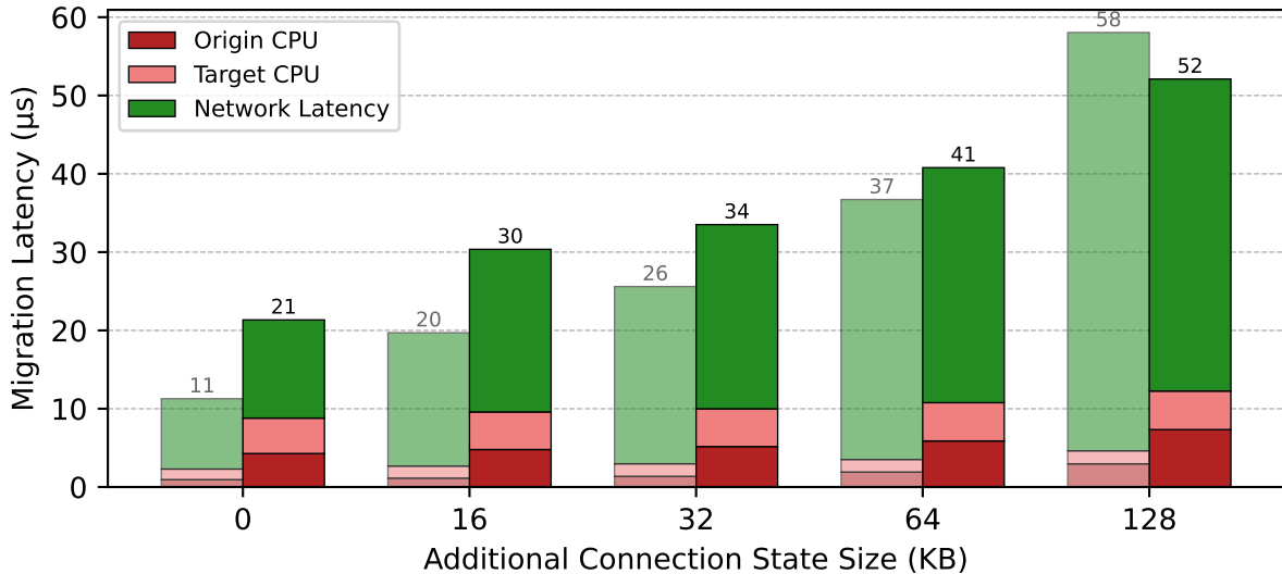
TCP migration latency by state size — paper (left, faded) vs ours (right)
