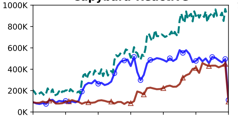
Capybara-Reactive
