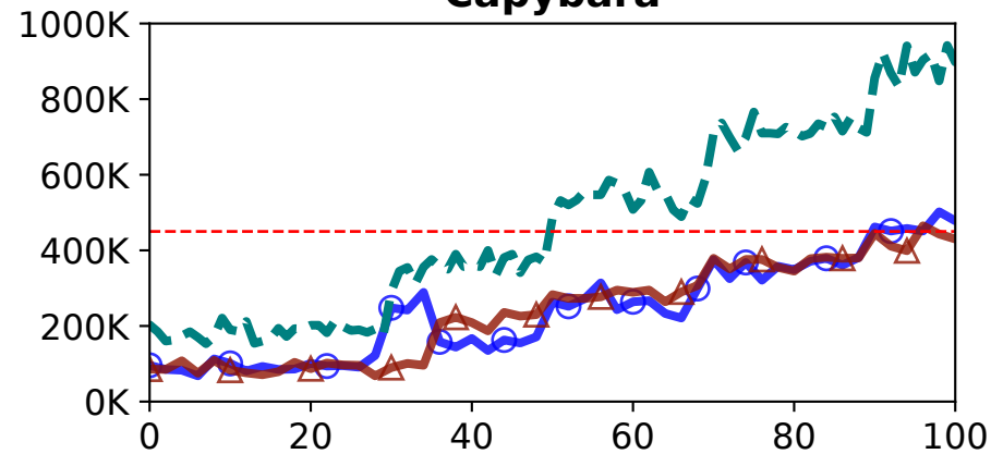
Capybara
