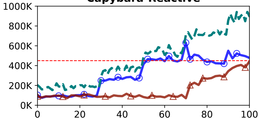
Capybara-Reactive
