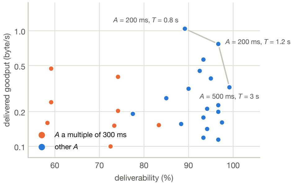
Figure 11: Delivered goodput against deliverability for all 26 conditions of the advertising-interval sweep at -24 dBm, both axes taken from the offline resweep. The line traces the Pareto frontier; note the logarithmic goodput axis.
