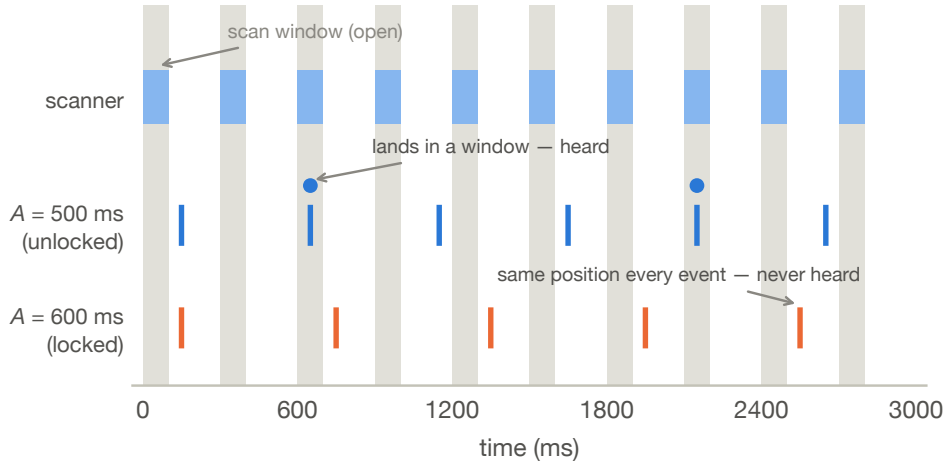
Figure 6: Schematic of the scan-cycle geometry (window width and starting offset are illustrative, not measured). The scanner opens a window once per 300 ms cycle. An advertiser at A = 600 ms revisits the same position on every event and, having started in the deaf gap, is never heard; an advertiser at A = 500 ms drifts across the cycle and is heard whenever an event lands inside a window.
