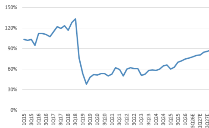
YAGEO low-end MLCC UTR trend
