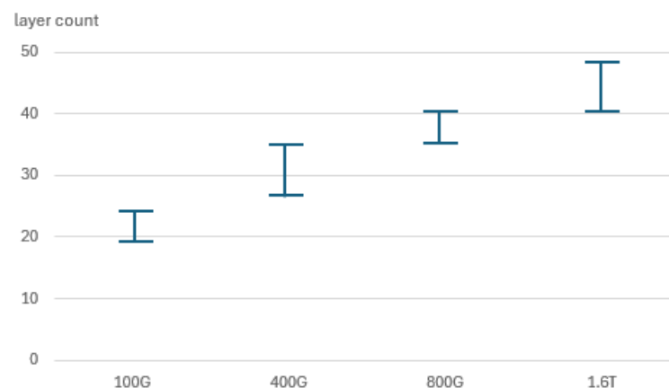
PCB layer count comparison (switch as illustration)
