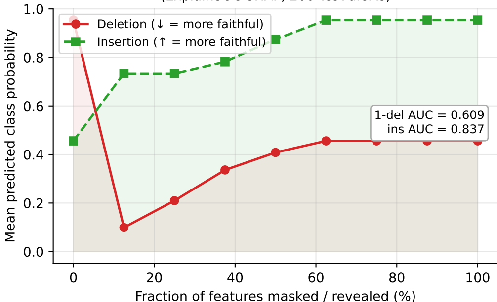
Deletion and Insertion Faithfulness Curves (ExplainSOC SHAP, 200 test alerts)
