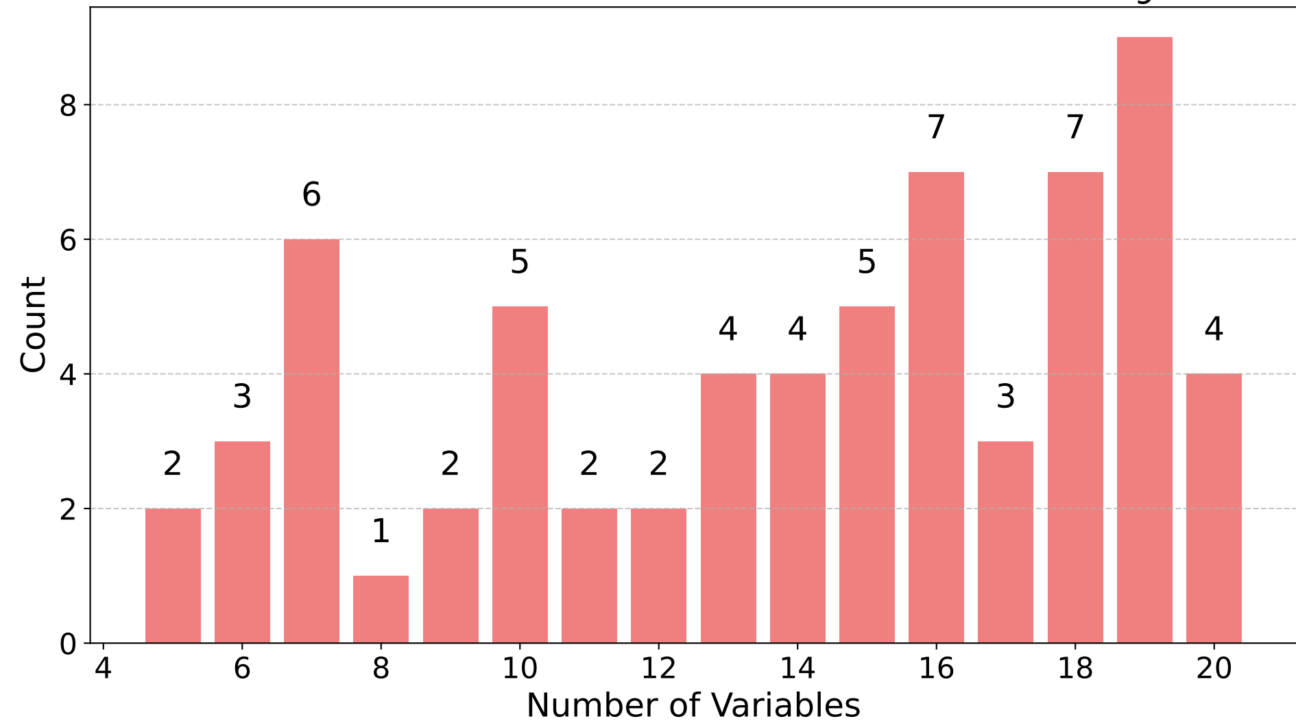
Distribution of BN Dimensions
