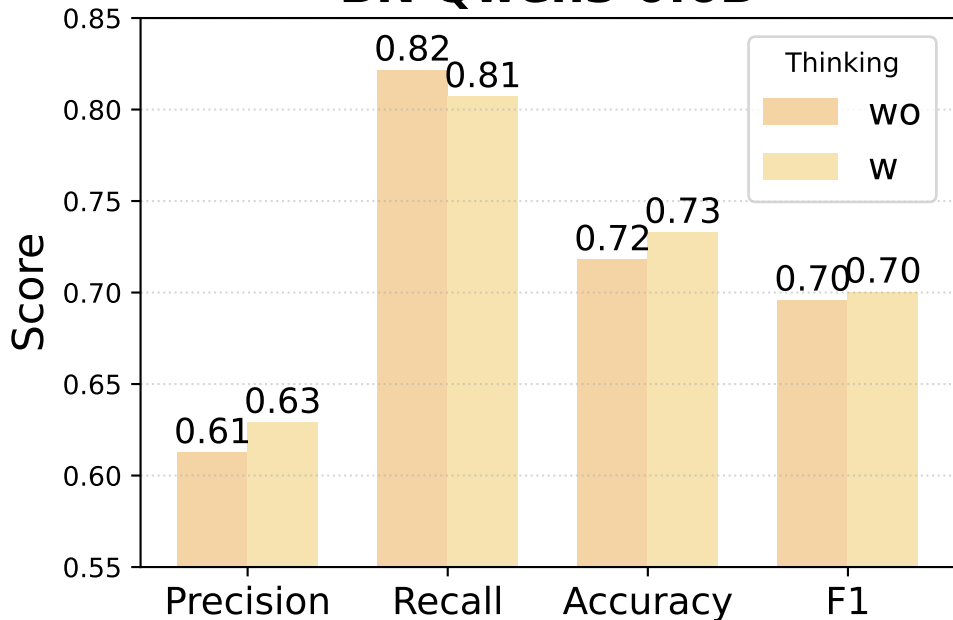
BN Qwen3 0.6B
