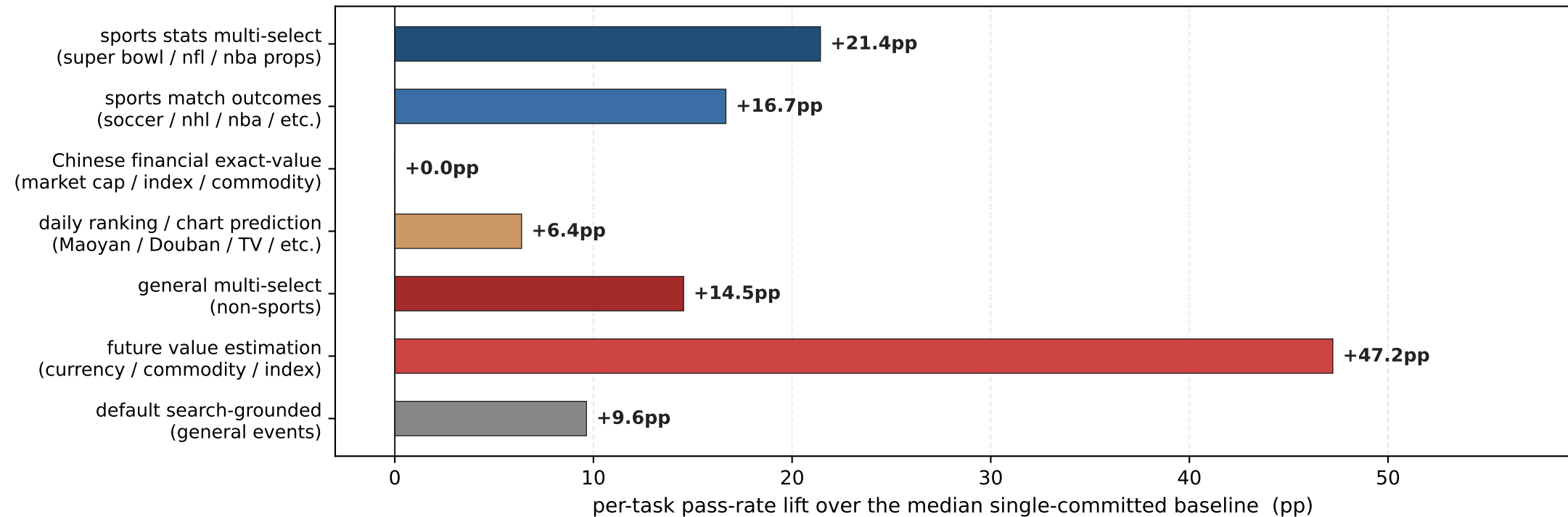
FutureX L_{\text{adapt}} evidence: per-branch lift of the routed harness over the median single-committed baseline. Each row = task type the navigation evolver spawned a dedicated skill for.
