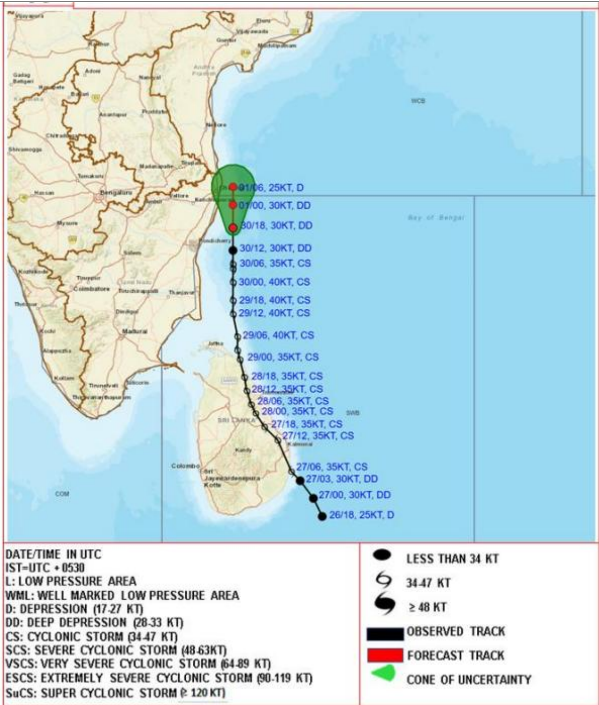
Figure- Deep Depression's Track. Source: RSMC
