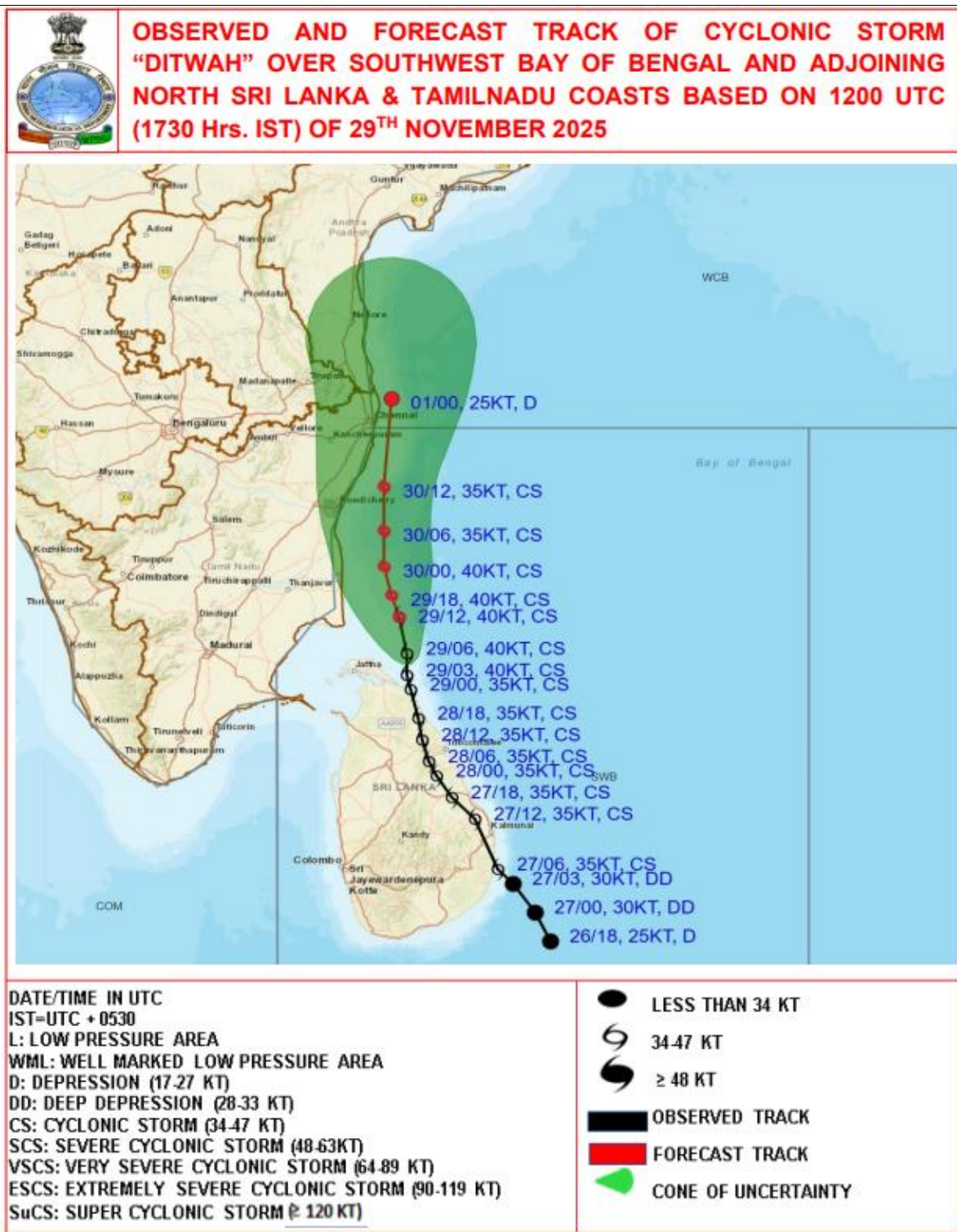
Figure- Cyclone Track of “Ditwah”. Source: RSMC
