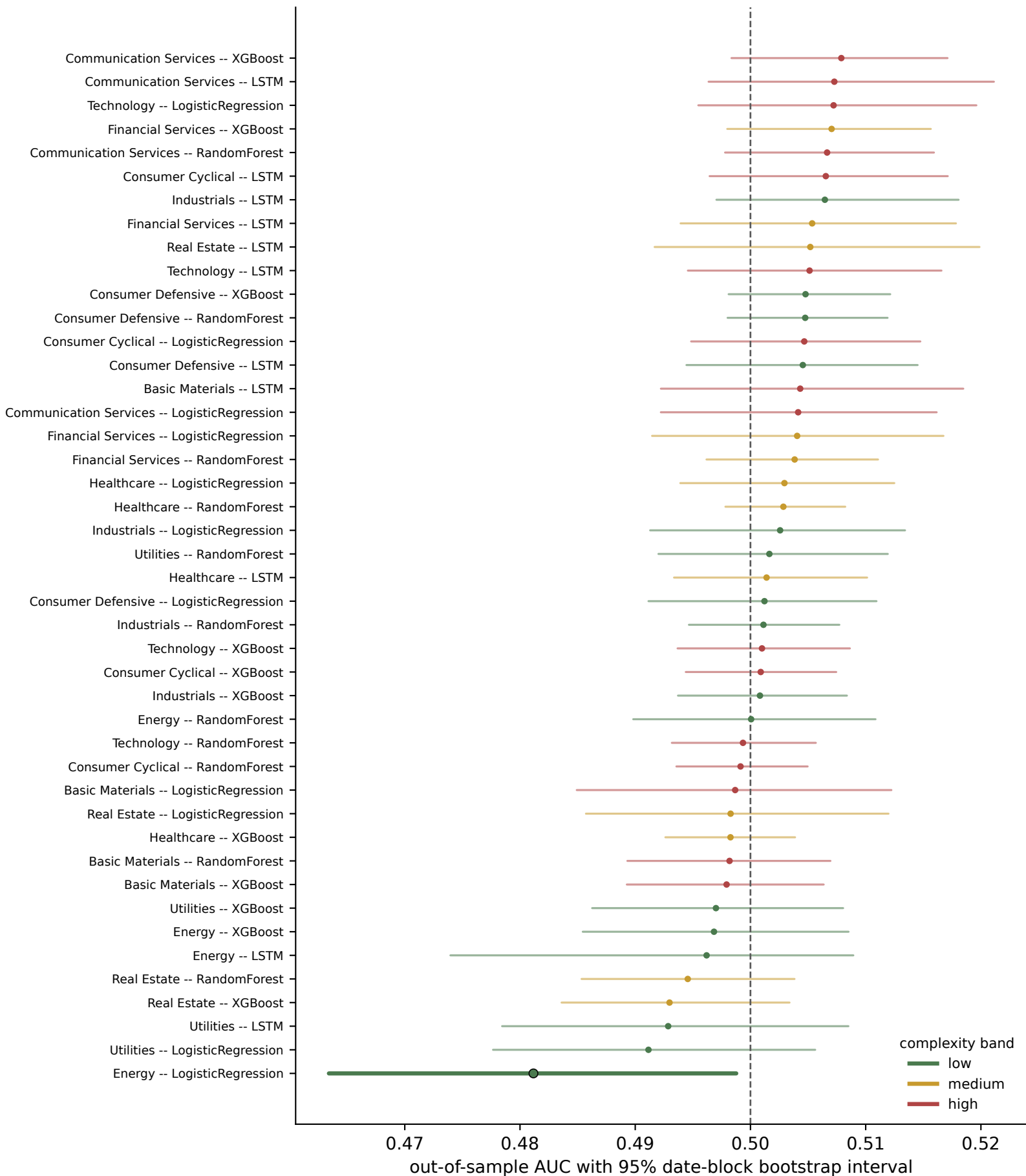
AUC and uncertainty for all 44 model-sector cells (1 intervals exclude 0.5; heavier lines)
