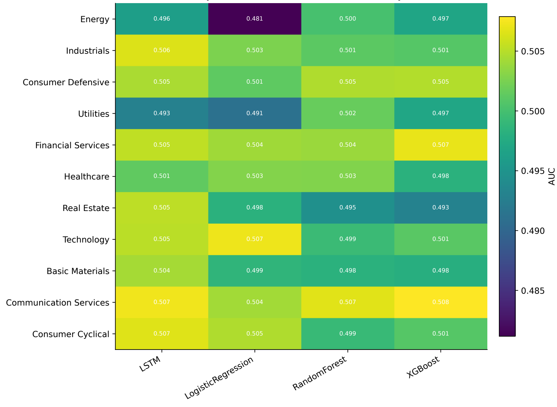
AUC by model and sector (sectors ordered by SCI)
