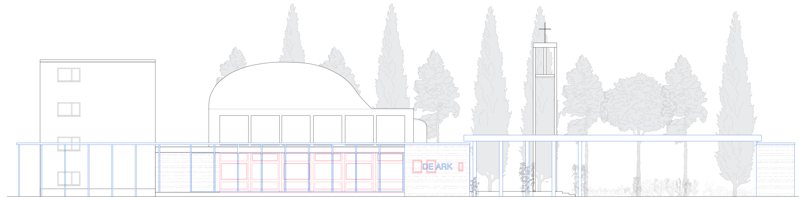
SOUTH FACADE ELEVATION 1:200
