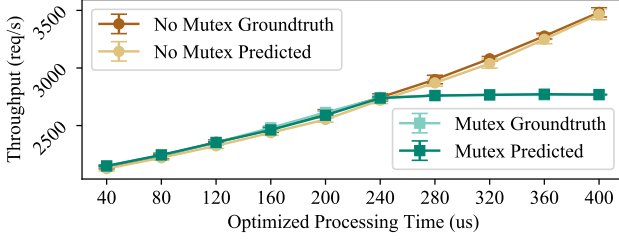
Figure 11: Throughput Prediction with Mutex Bottleneck
