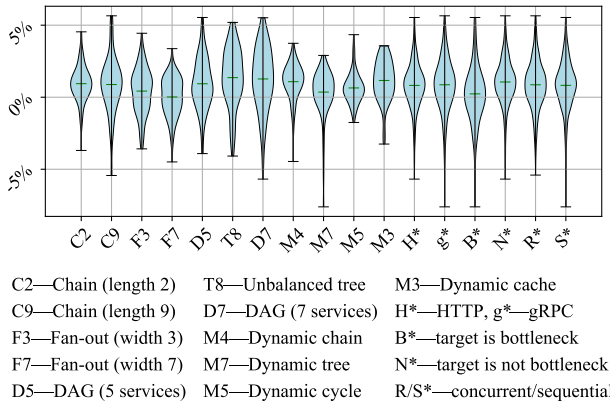
Figure 10: Prediction errors for synthetic experiments grouped by different characteristics. The green line indicates the mean.
