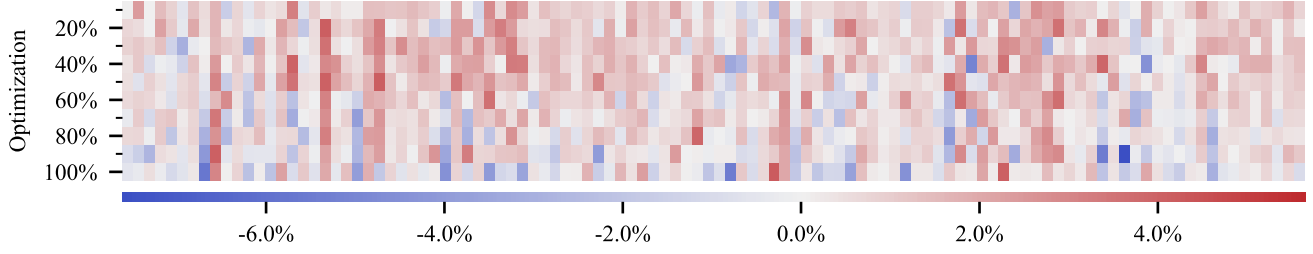
Figure 9: Error heatmap of SLOWPOKE across all synthetic call graph configurations. Each row represents a single callgraph combination, and each cell indicates the estimation error for a specific optimization percentage (10%–100%), where a 50% optimization indicates a 50% reduction of target service’s average processing time per request. The intensity of the color corresponds to the magnitude of the error. Red blocks denote over-estimation while blue indicates under-estimation.
