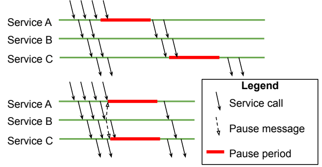
Figure 6: Uncoordinated (top) vs. Coordinated (bottom) pausing.
