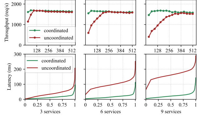
Figure 14: Top row: Throughput measured with varying connection parameter in wrk . The applications have simple chain topology with 3, 6, and 9 services. Bottom row: Latency at different percentile with the same set of applications.
