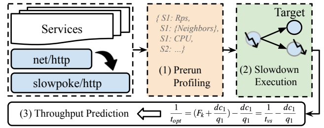
Figure 1: SLOWPOKE Overview. Given a microservice application importing SLOWPOKE’s augmented libraries running on Kubernetes, SLOWPOKE (1) pre-runs experiments to collect per-service information; (2) measures performance while selectively slowing down non-target services; and (3) applies a performance model to quantify throughput improvements.
