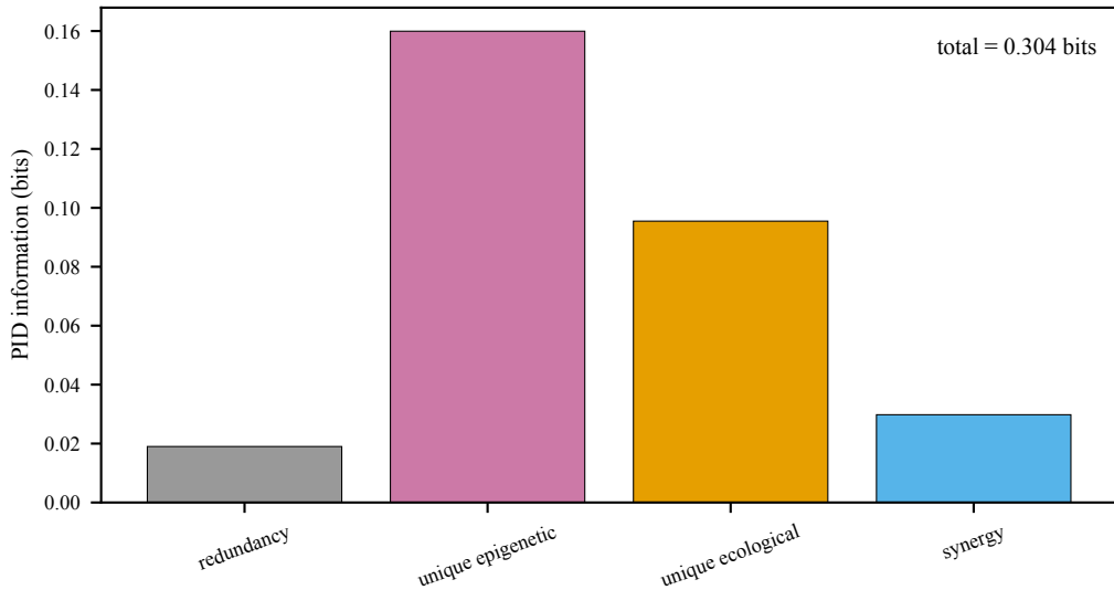
Partial information decomposition of epigenetic and ecological contributions
