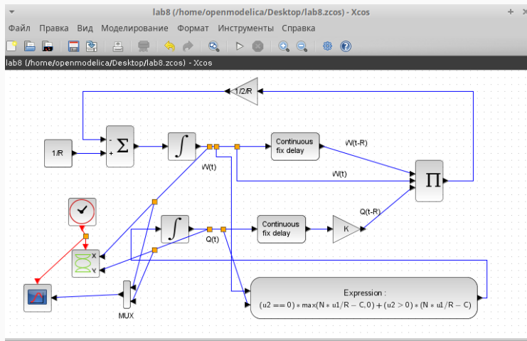
. 2: TCP/AQM xcos
