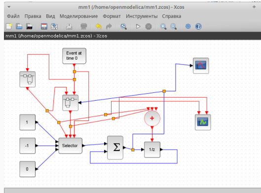
. 4: M|M|1|_{\infty} xcos
