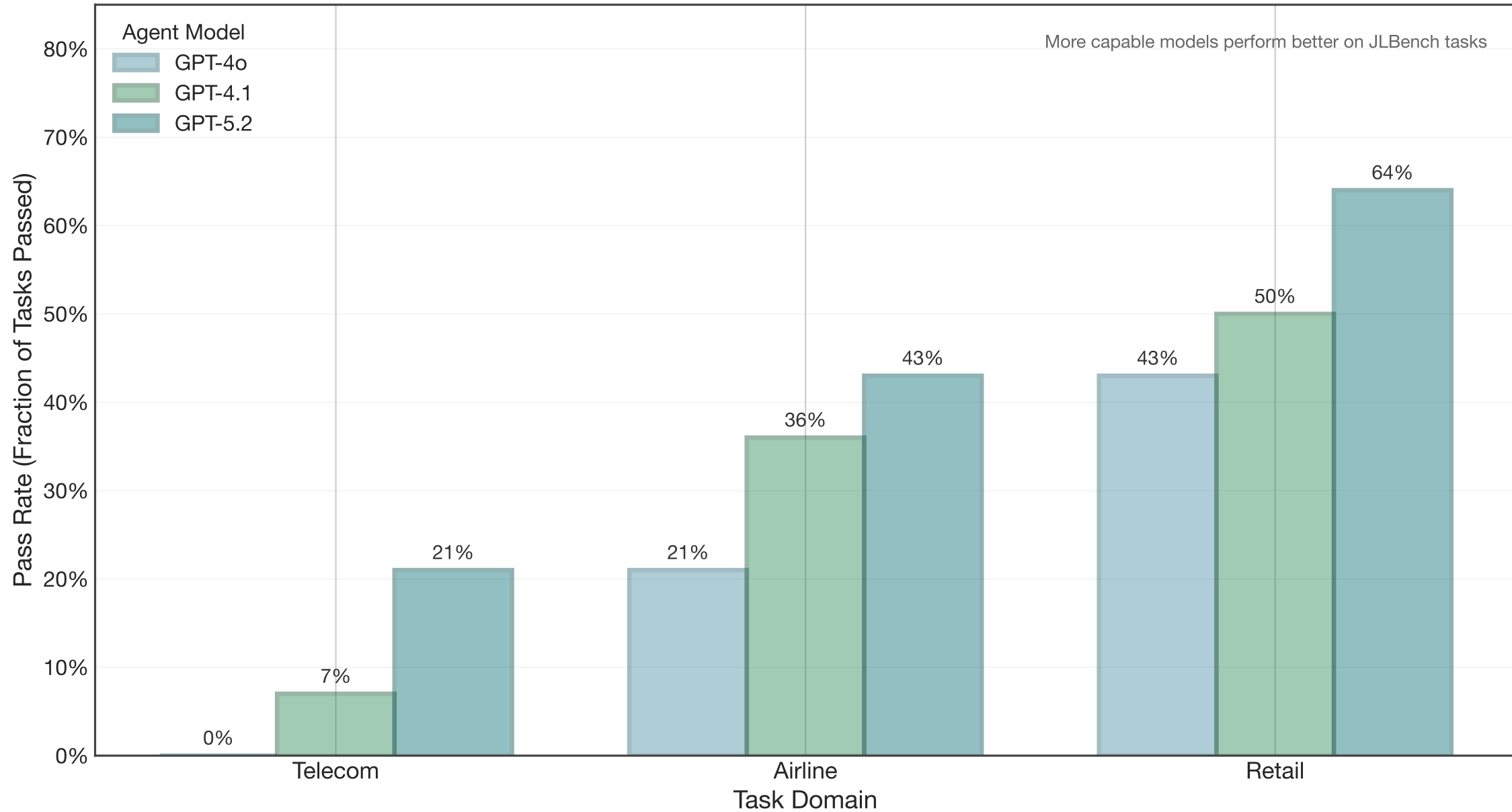
Task-Agent Performance by Model and Domain on JLBench Tasks
