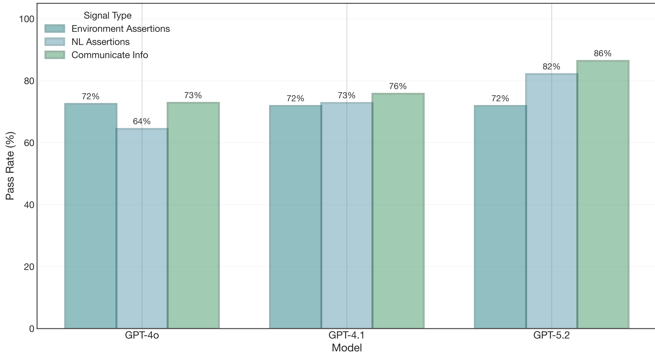
Partial Evaluation Signals on JLBench Tasks by Task-Agent Capability
